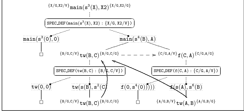
Fig. 2. Analysis Graph computed by ABS.INT_WITH_SPEC_DEF
