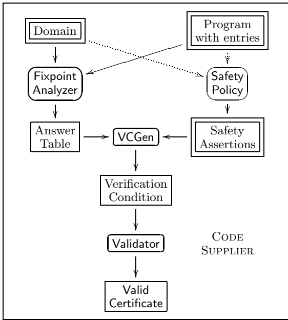
Figure 1: Abstract Interpretation-based Mobile Code Certification in CiaoPP
